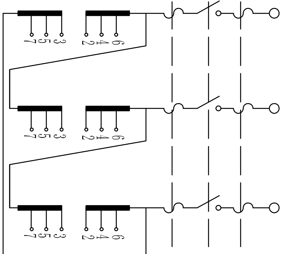
SCHEMATIC DIAGRAM
